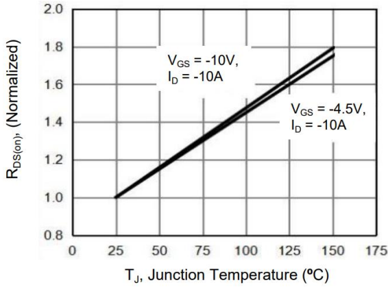
Figure 7. Drain-Source On-Resistance
