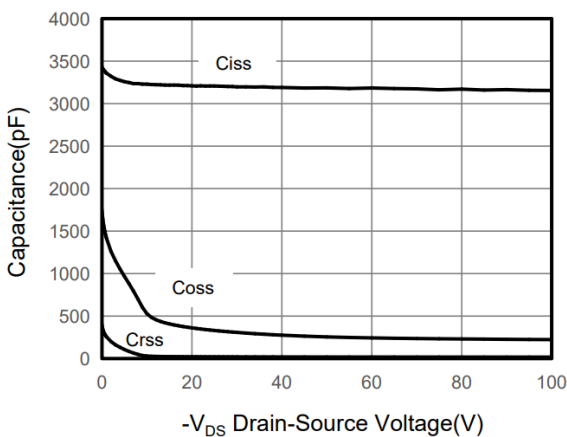
Figure 5. Capacitance
