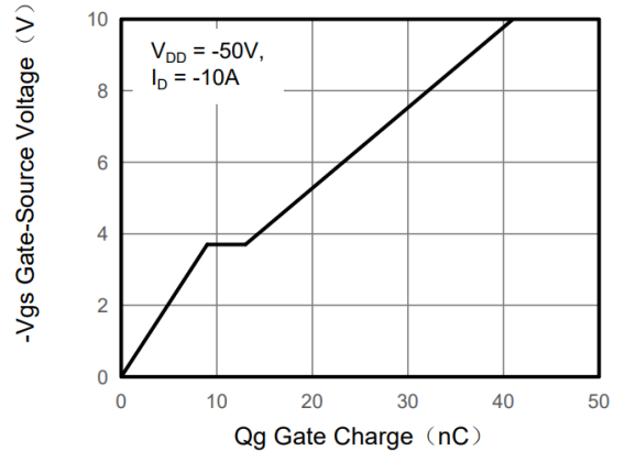
Figure 4. Gate Charge
