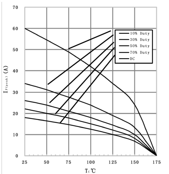
3) Current Derating
