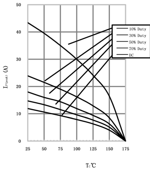
3) Current Derating
