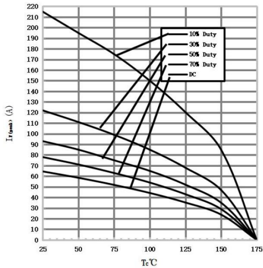
3) Current Derating
