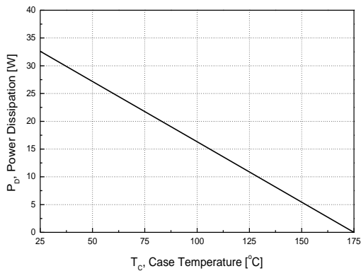
Figure 3. Power Dissipation
