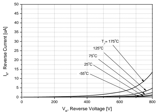
Figure 2. Reverse Characteristics
