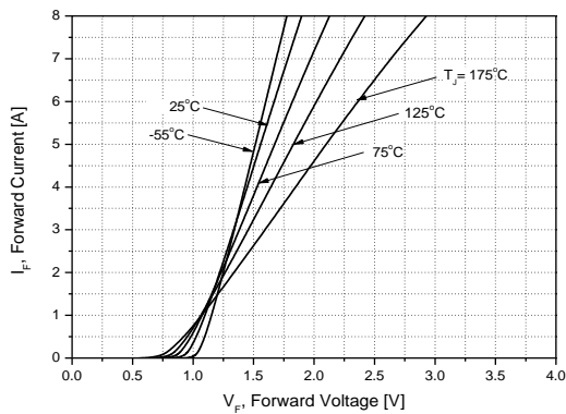
Figure 1. Forward Characteristics
