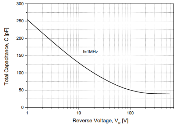
Figure 8. Total Capacitance
