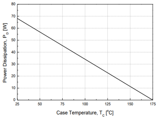
Figure 3. Power Dissipation
