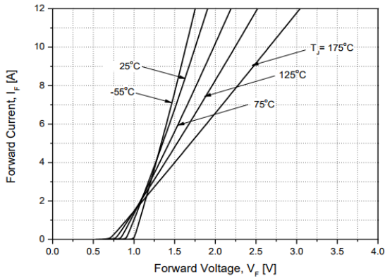
Figure 1. Forward Characteristics
