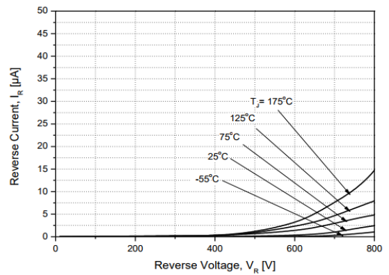
Figure 2. Reverse Characteristics
