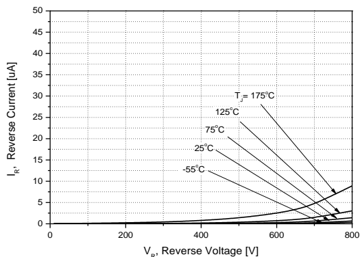
Figure 2. Reverse Characteristics
