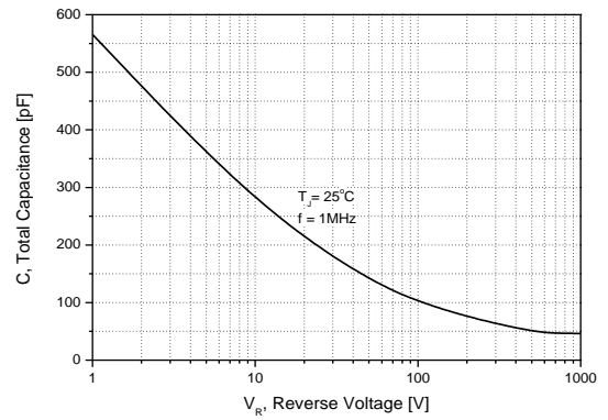
Figure 8. Total Capacitance
