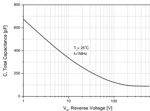
Figure 8. Total Capacitance
