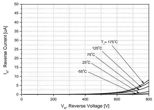
Figure 2. Reverse Characteristics
