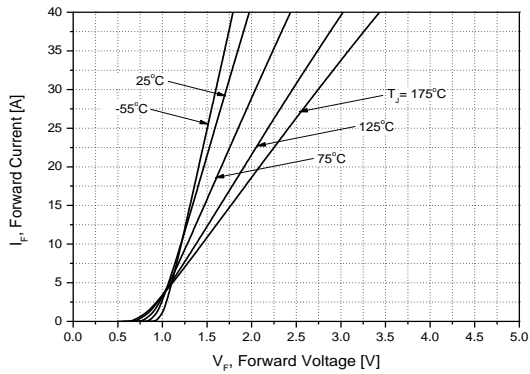
Figure 1. Forward Characteristics
