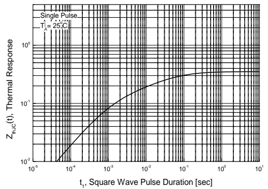
Figure 4. Transient Thermal Resistance
