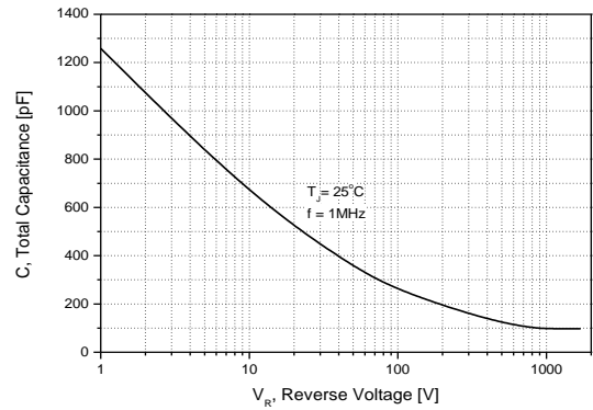
Figure 8. Total Capacitance
