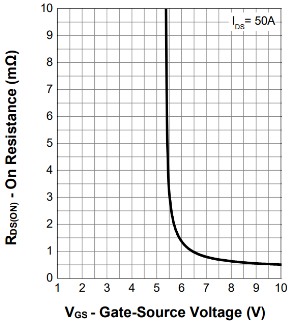
Figure 7. Transfer Characteristics
