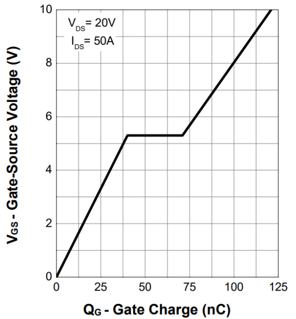
Figure 12. Gate Charge
