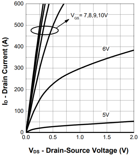
Figure 5. Output Characteristics
