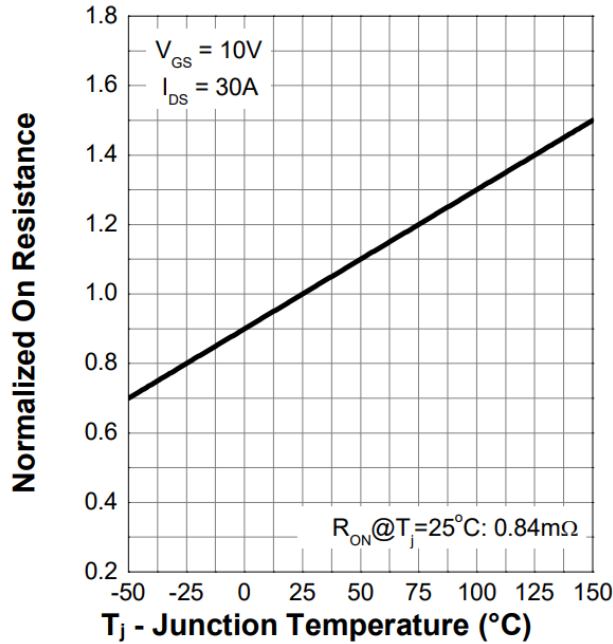
Figure 9. Normalized On-Resistance
