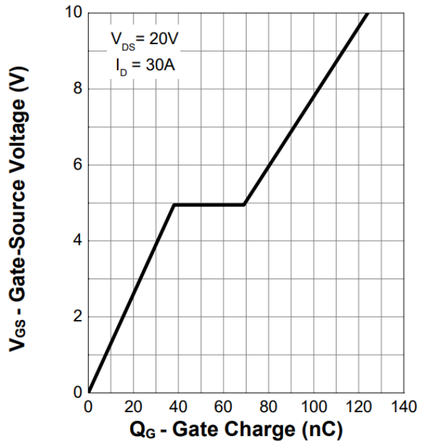
Figure 12. Gate Charge
