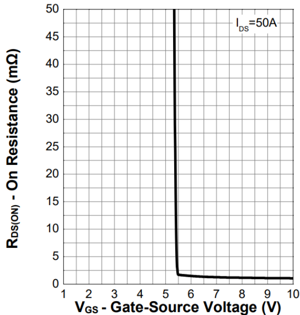
Figure 7. Transfer Characteristics
