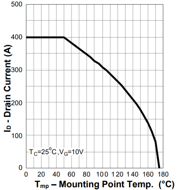
Figure 2. Current Capability
