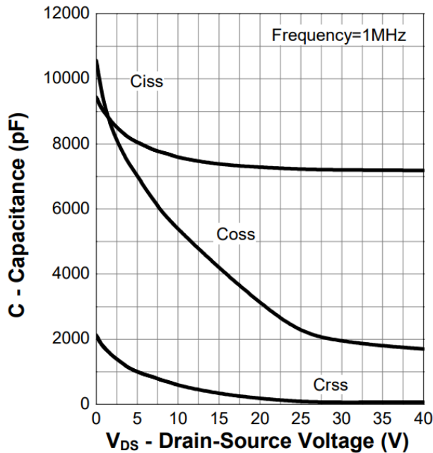
Figure 11. Capacitance
