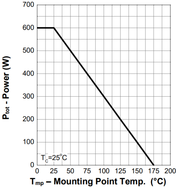
Figure 1. Power Capability
