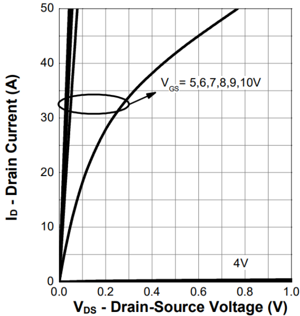
Figure 5. Output Characteristics
