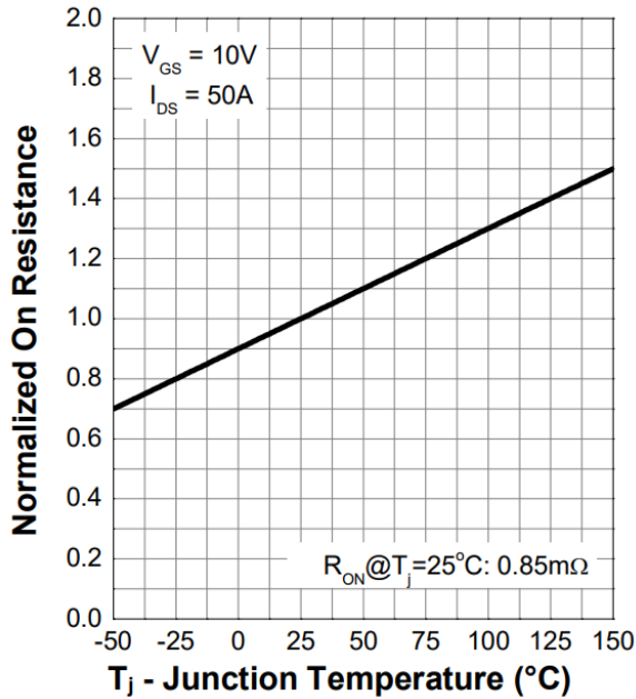
Figure 9. Normalized On-Resistance
