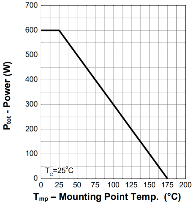
Figure 1. Power Capability
