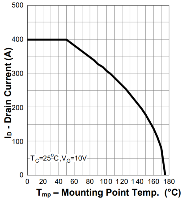
Figure 2. Current Capability
