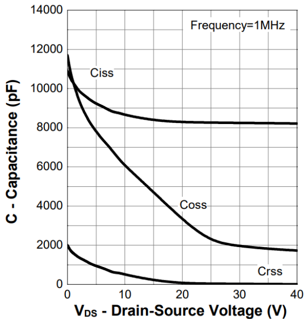
Figure 11. Capacitance
