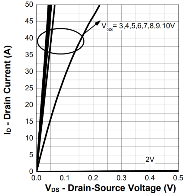
Figure 5. Output Characteristics
