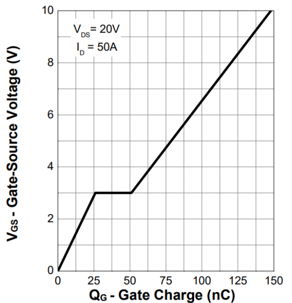
Figure 12. Gate Charge
