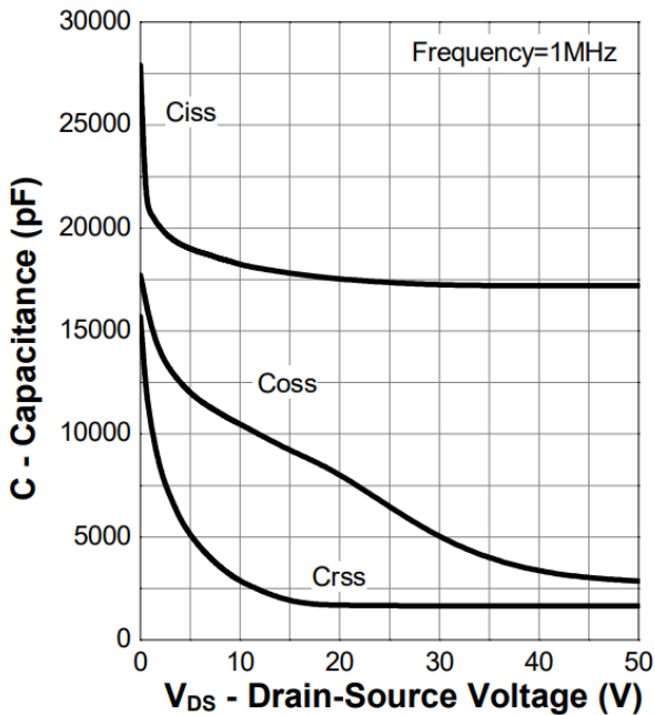
Figure 11. Capacitance
