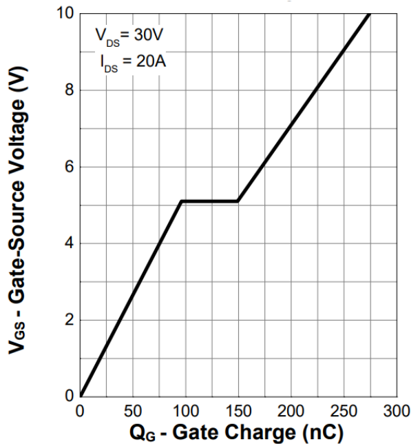
Figure 12. Gate Charge
