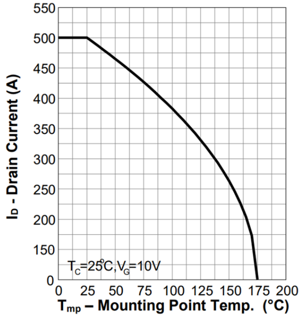
Figure 2. Current Capability
