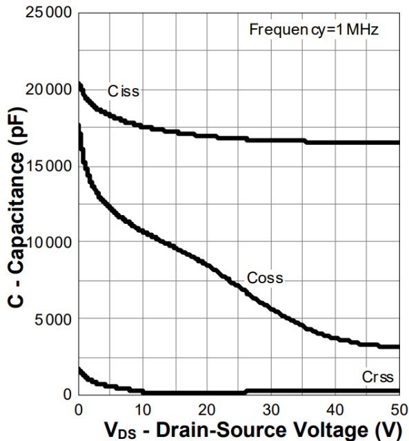
Figure 11. Capacitance
