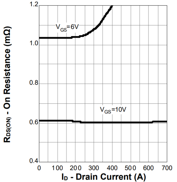
Figure 6. On-Resistance
