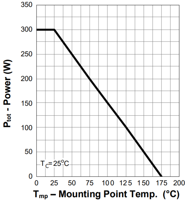
Figure 1. Power Capability
