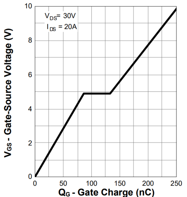
Figure 12. Gate Charge
