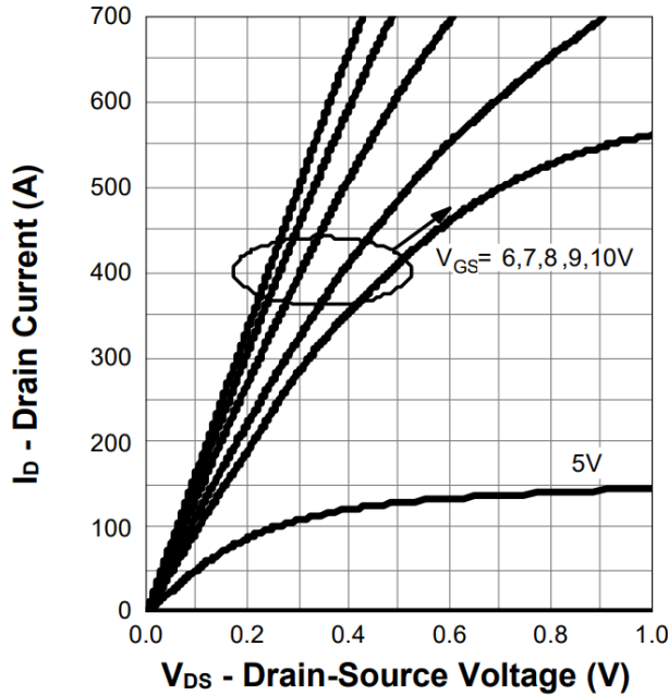
Figure 5. Output Characteristics
