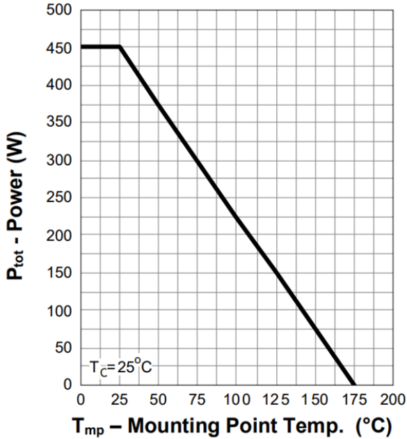
Figure 1. Power Capability
