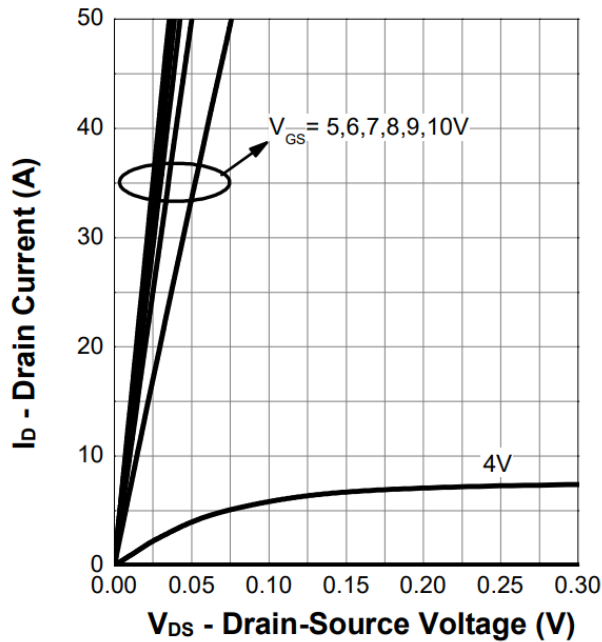
Figure 5. Output Characteristics
