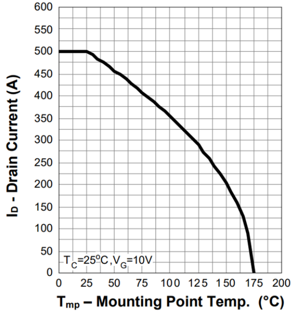
Figure 2. Current Capability
