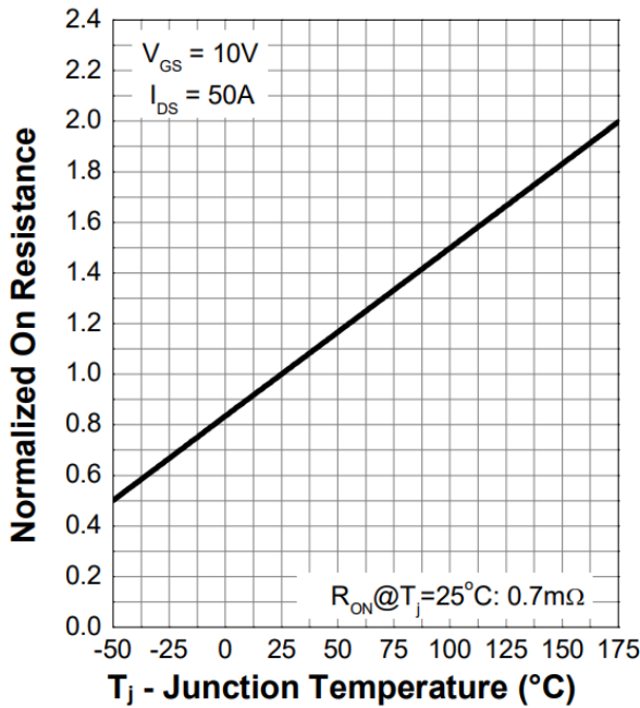
Figure 9. Normalized On-Resistance
