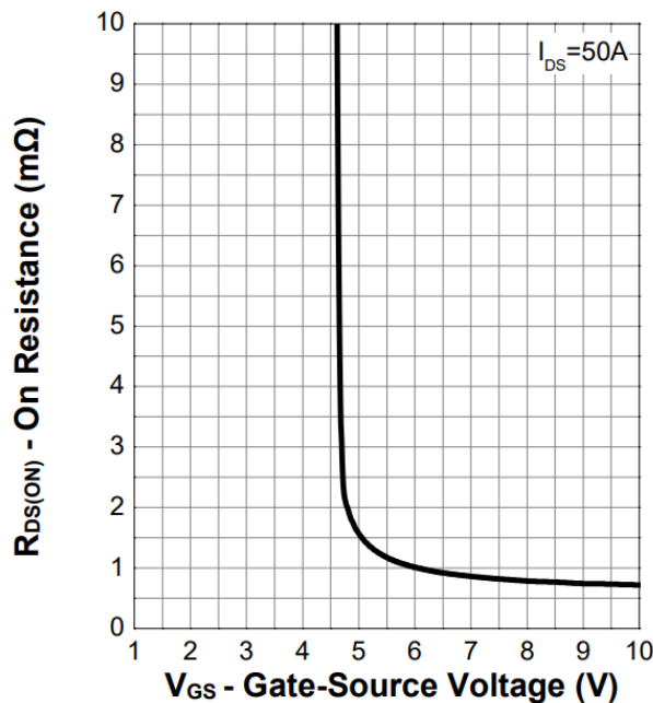
Figure 7. Transfer Characteristics
