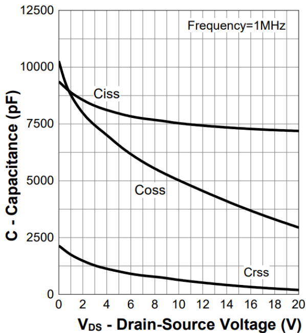
Figure 11. Capacitance
