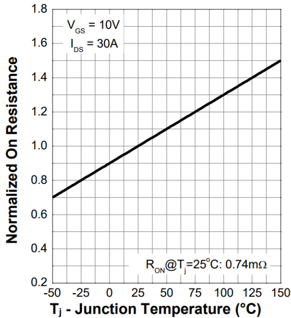
Figure 9. Normalized On-Resistance
