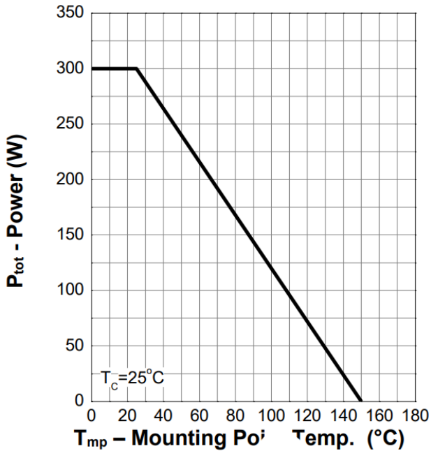
Figure 1. Power Capability
