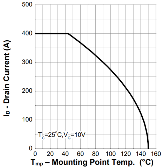
Figure 2. Current Capability
