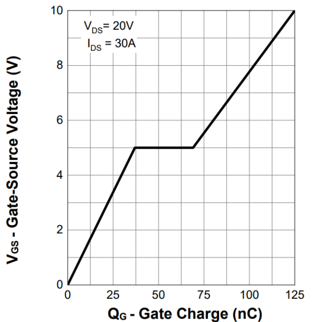
Figure 12. Gate Charge
