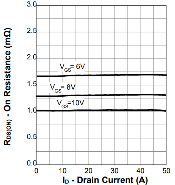
Figure 6. On-Resistance
