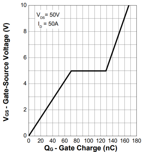
Figure 12. Gate Charge
