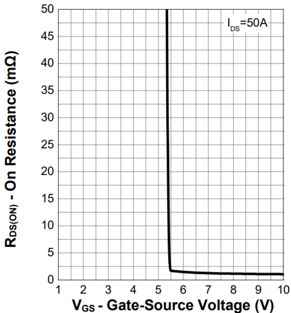
Figure 7. Transfer Characteristics
