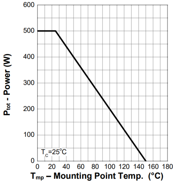
Figure 1. Power Capability
