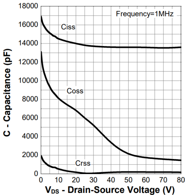
Figure 11. Capacitance
