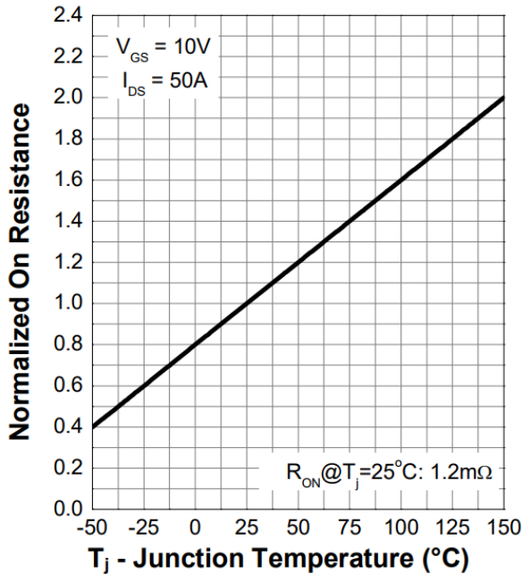
Figure 9. Normalized On-Resistance
