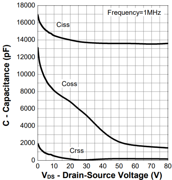
Figure 11. Capacitance
