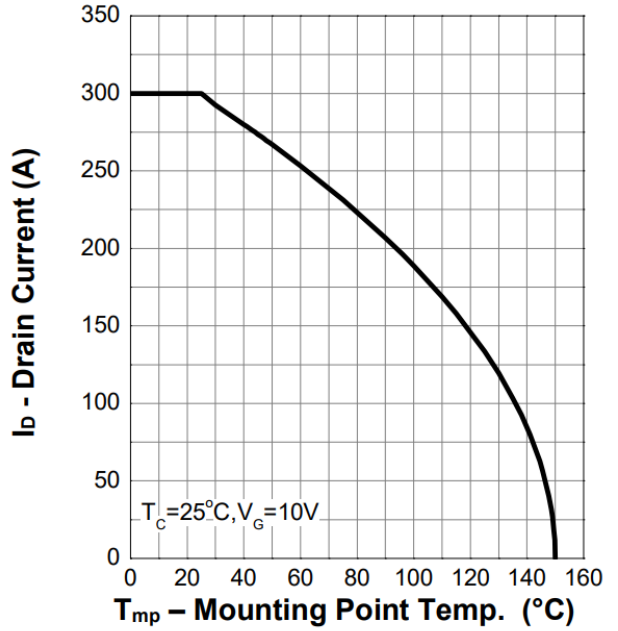
Figure 2. Current Capability
