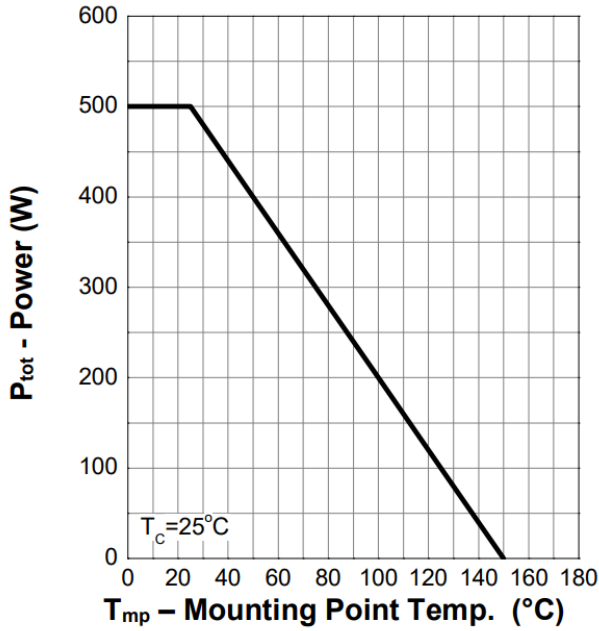
Figure 1. Power Capability
