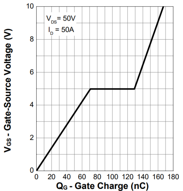
Figure 12. Gate Charge
