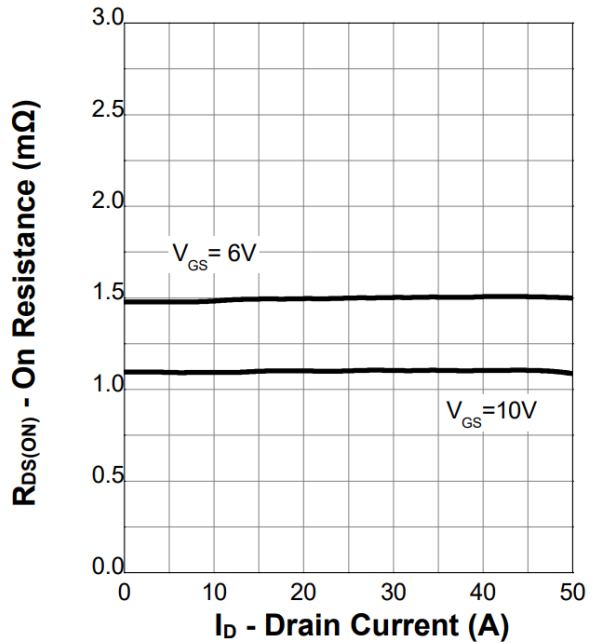
Figure 6. On-Resistance
