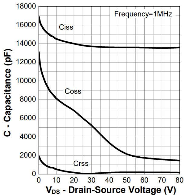
Figure 11. Capacitance
