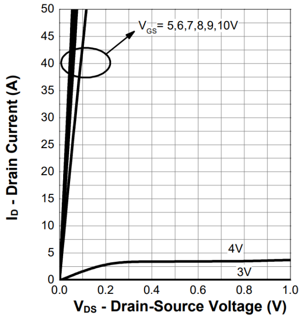
Figure 5. Output Characteristics
