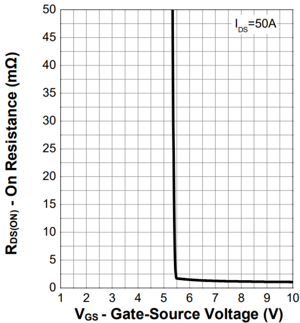
Figure 7. Transfer Characteristics
