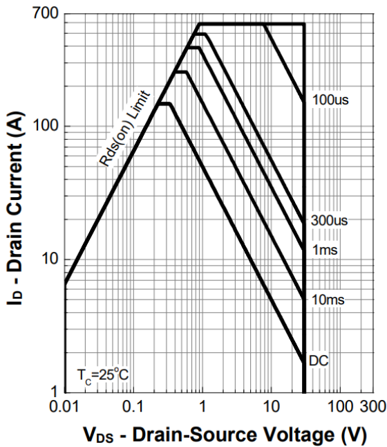
Figure 3. Safe Operating Area
