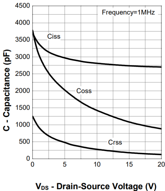
Figure 11. Capacitance
