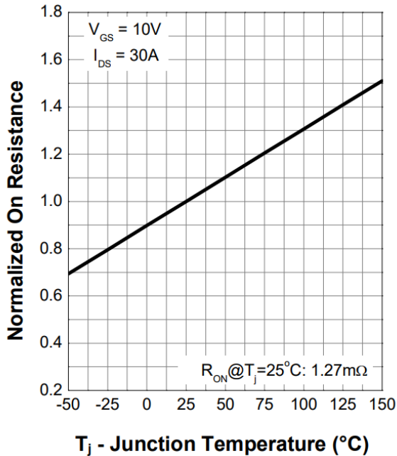
Figure 9. Normalized On-Resistance
