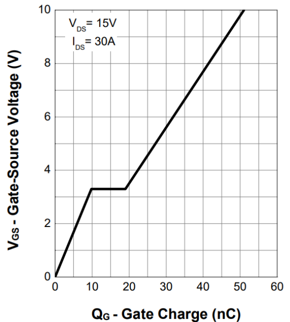
Figure 12. Gate Charge
