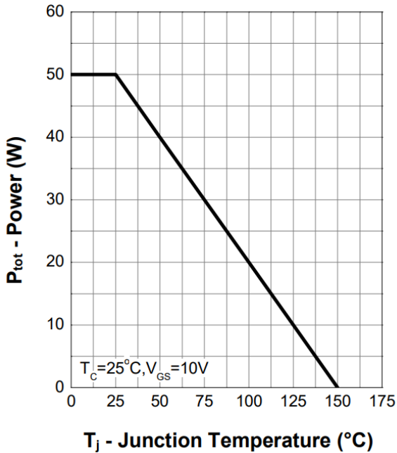
Figure 1. Power Capability
