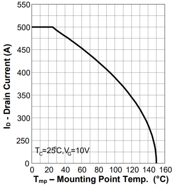
Figure 2. Current Capability
