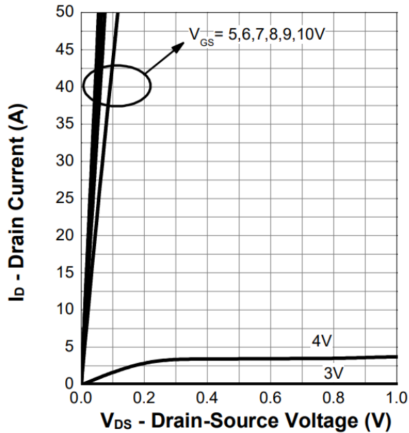
Figure 5. Output Characteristics
