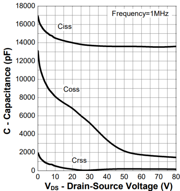
Figure 11. Capacitance
