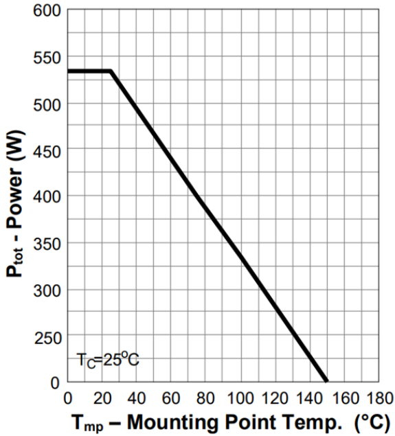
Figure 1. Power Capability
