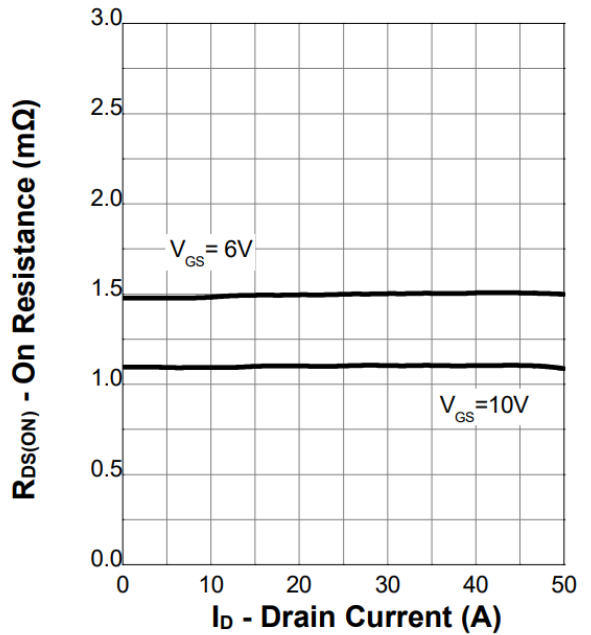
Figure 6. On-Resistance
