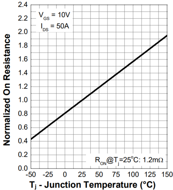
Figure 9. Normalized On-Resistance
