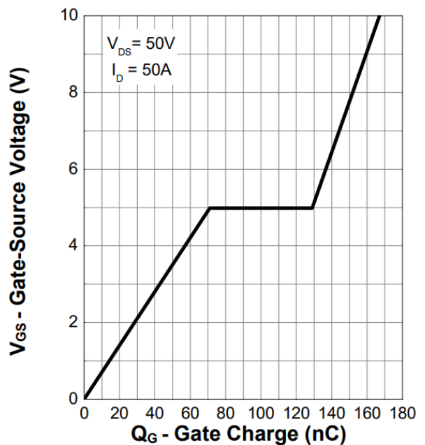
Figure 12. Gate Charge
