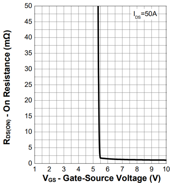
Figure 7. Transfer Characteristics
