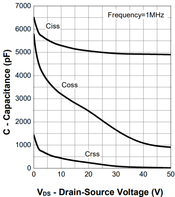
Figure 11. Capacitance
