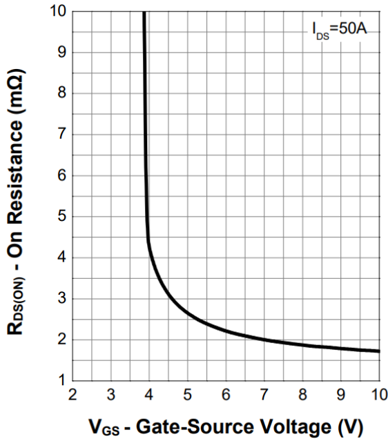
Figure 7. Transfer Characteristics
