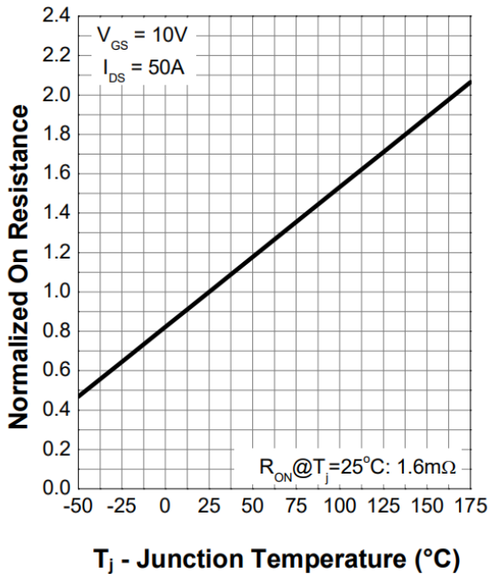
Figure 9. Normalized On-Resistance
