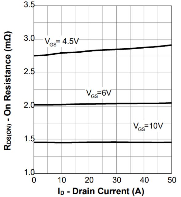
Figure 6. On-Resistance
