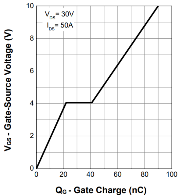
Figure 12. Gate Charge
