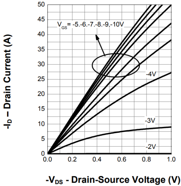
Figure 5. Output Characteristics
