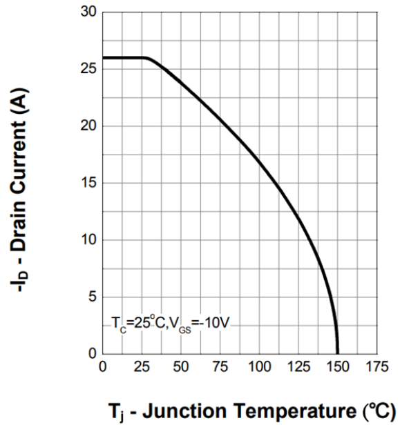
Figure 2. Current Capability
