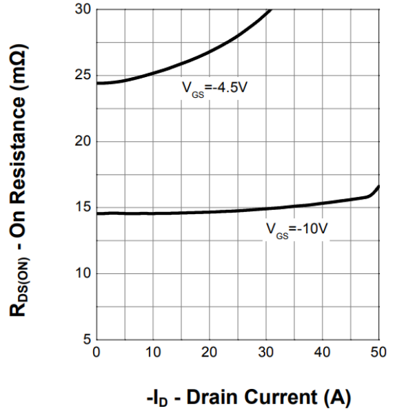
Figure 6. On-Resistance
