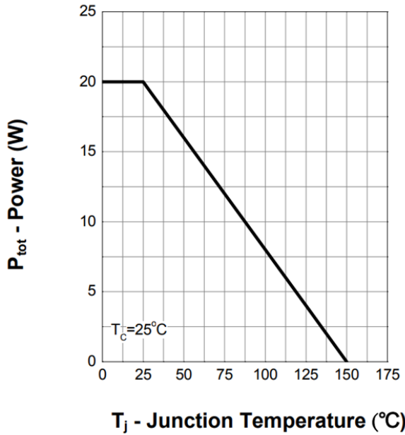
Figure 1. Power Capability
