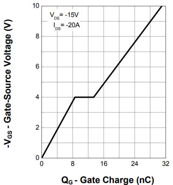
Figure 12. Gate Charge
