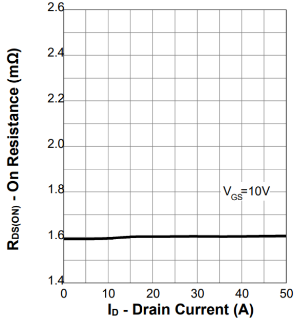
Figure 6. On-Resistance
