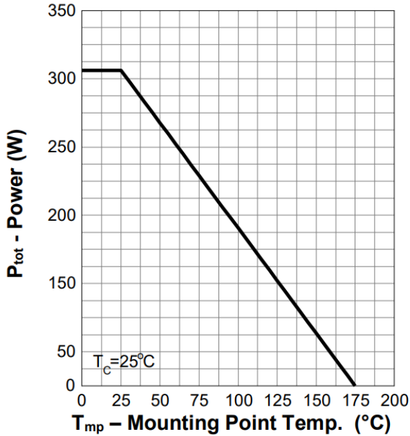
Figure 1. Power Capability
