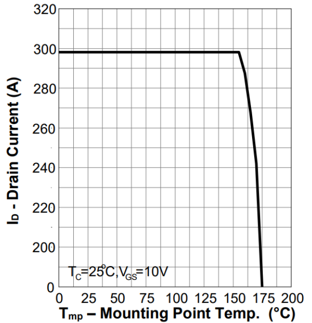
Figure 2. Current Capability
