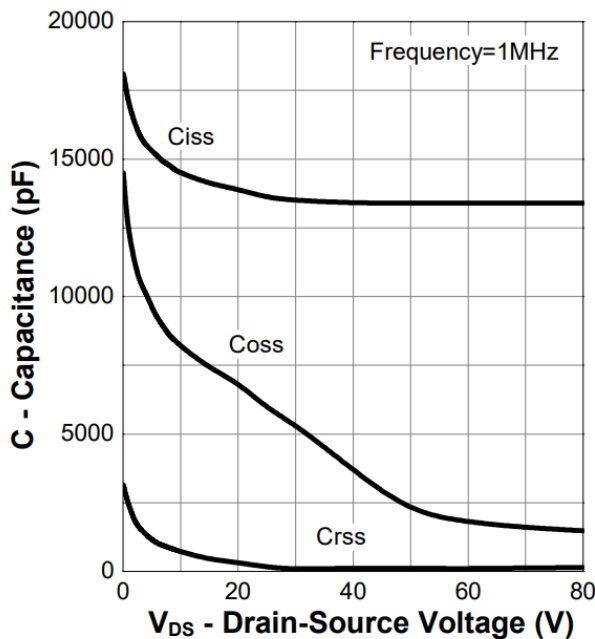
Figure 11. Capacitance
