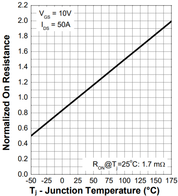
Figure 9. Normalized On-Resistance
