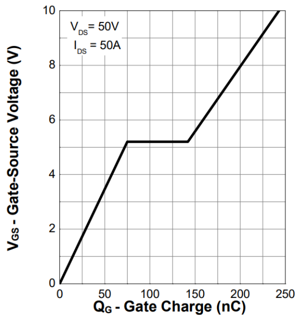
Figure 12. Gate Charge
