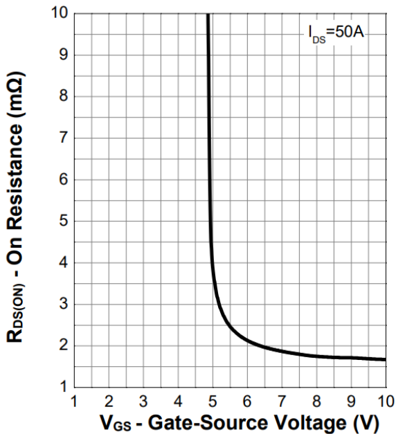
Figure 7. Transfer Characteristics
