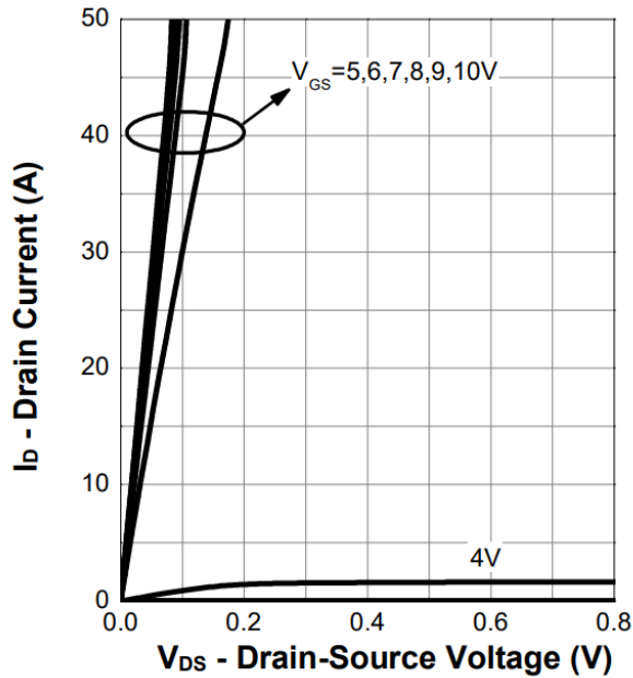
Figure 5. Output Characteristics
