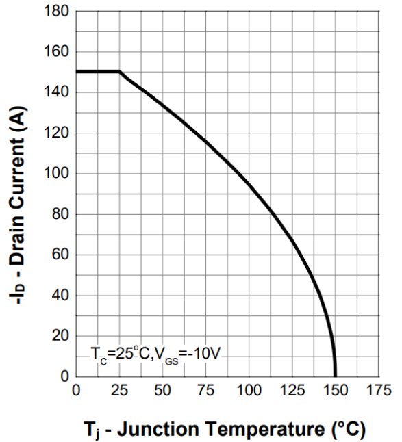
Figure 2. Current Capability
