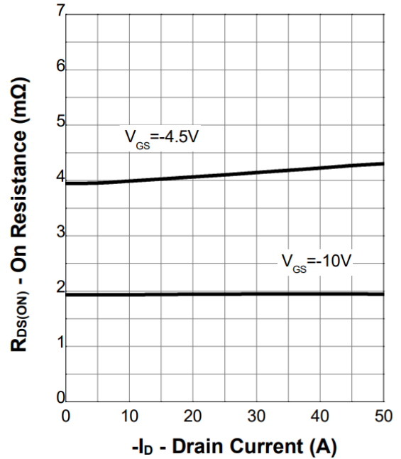
Figure 6. On-Resistance
