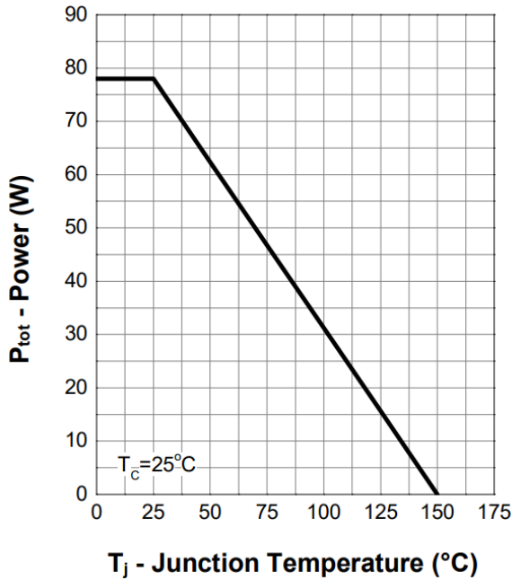
Figure 1. Power Capability
