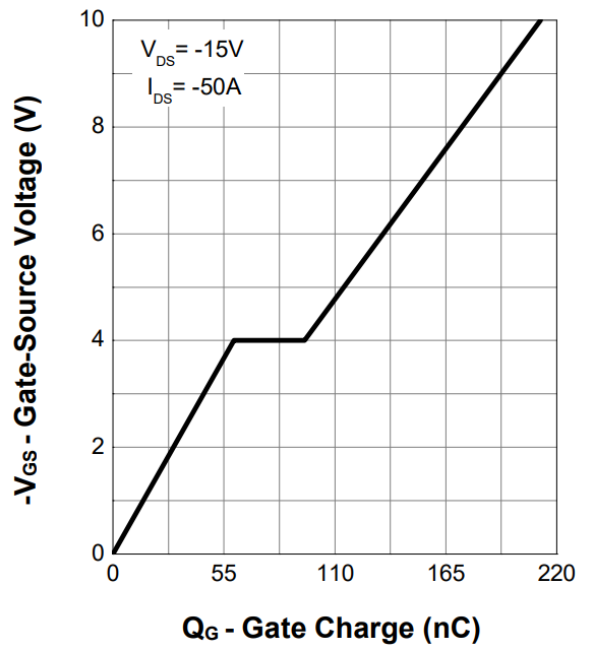
Figure 12. Gate Charge
