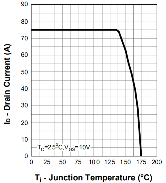
Figure 2. Current Capability
