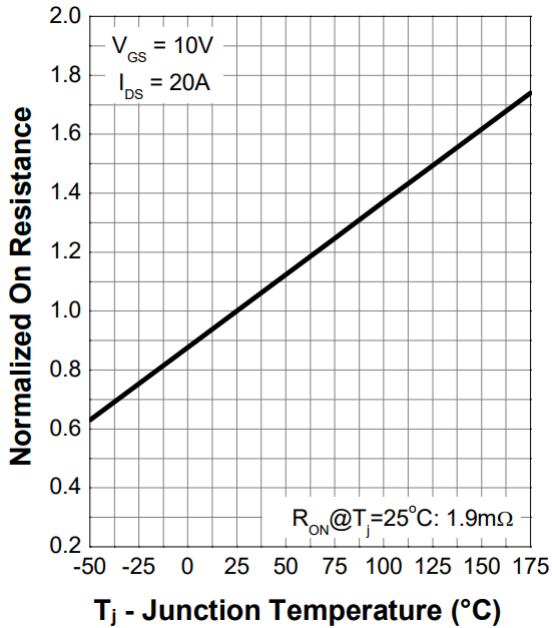
Figure 9. Normalized On-Resistance
