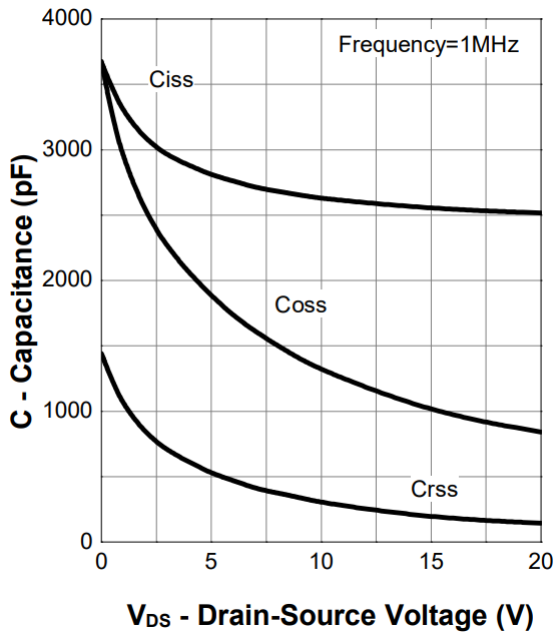
Figure 11. Capacitance
