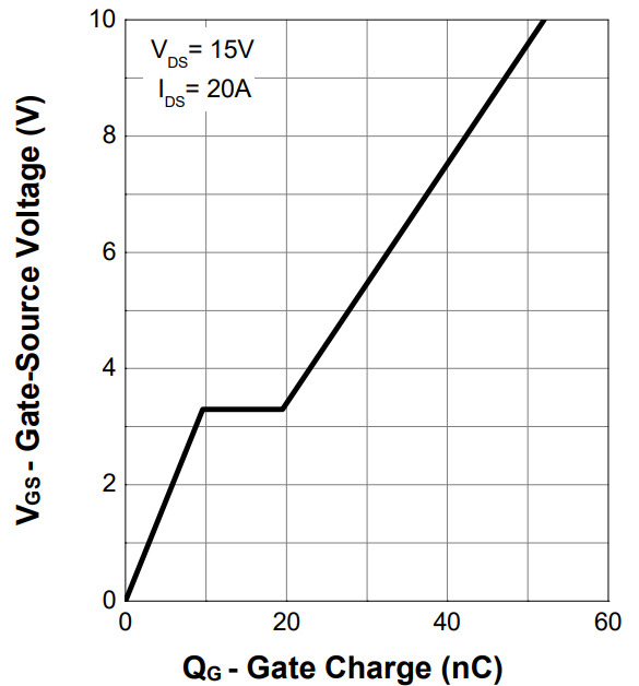
Figure 12. Gate Charge
