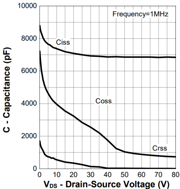
Figure 11. Capacitance
