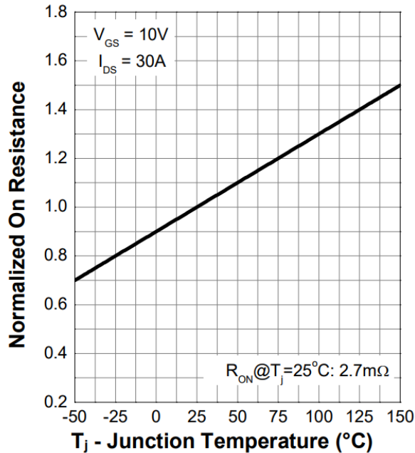
Figure 9. Normalized On-Resistance
