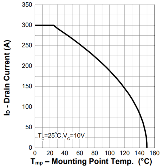
Figure 2. Current Capability
