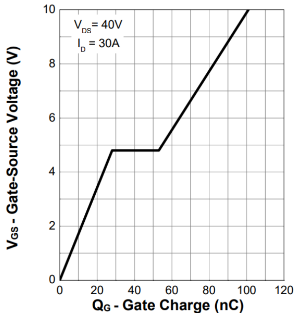
Figure 12. Gate Charge
