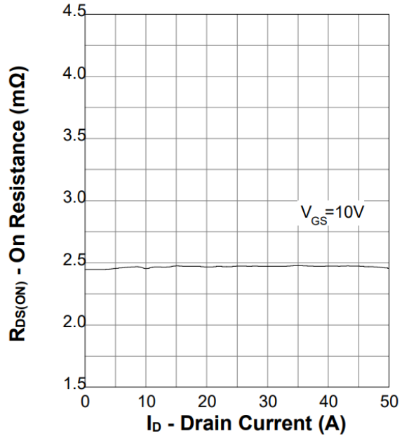
Figure 6. On-Resistance
