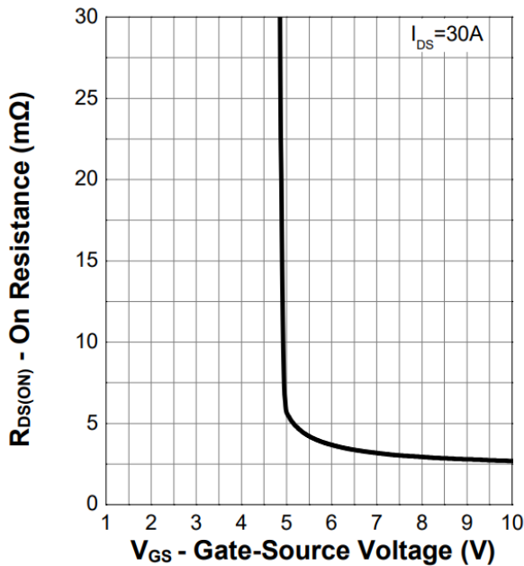
Figure 7. Transfer Characteristics
