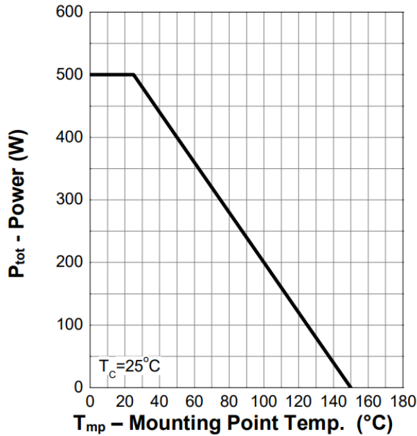
Figure 1. Power Capability
