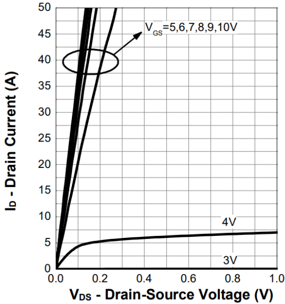
Figure 5. Output Characteristics
