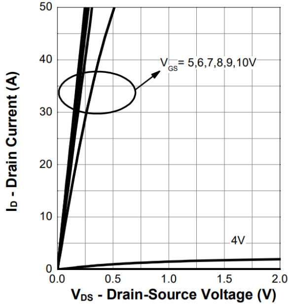
Figure 5. Output Characteristics
