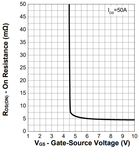
Figure 7. Transfer Characteristics
