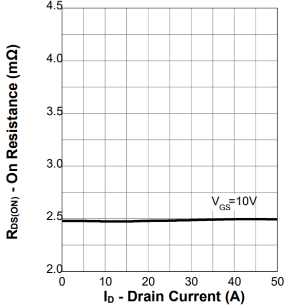
Figure 6. On-Resistance
