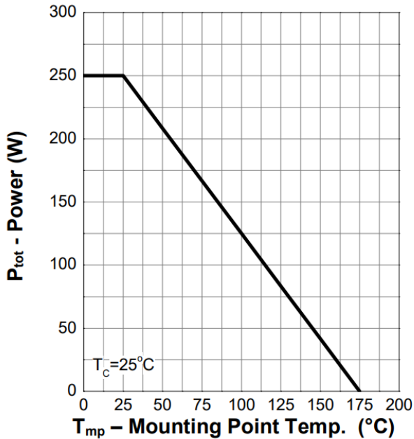
Figure 1. Power Capability
