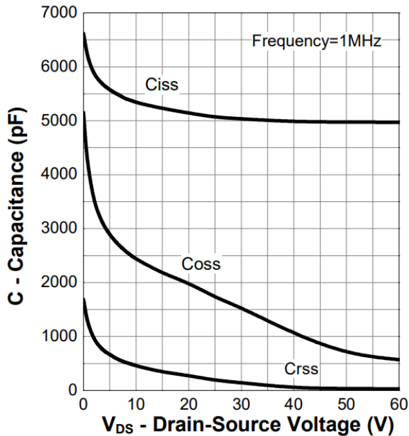
Figure 11. Capacitance
