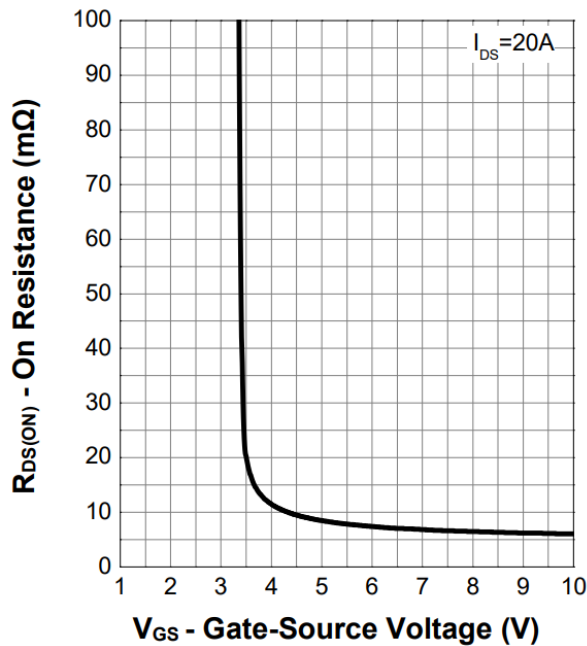
Figure 7. Transfer Characteristics
