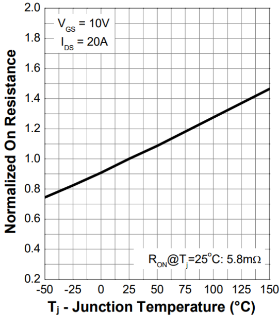
Figure 9. Normalized On-Resistance
