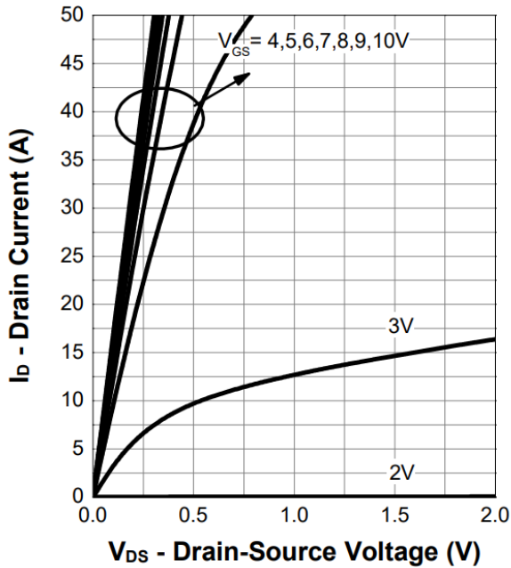
Figure 5. Output Characteristics
