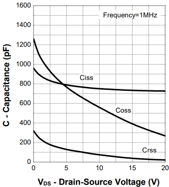
Figure 11. Capacitance
