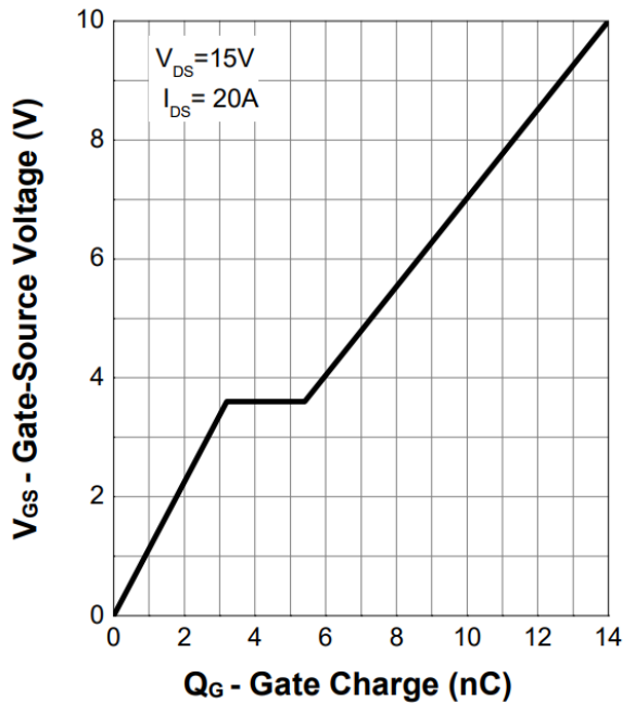
Figure 12. Gate Charge
