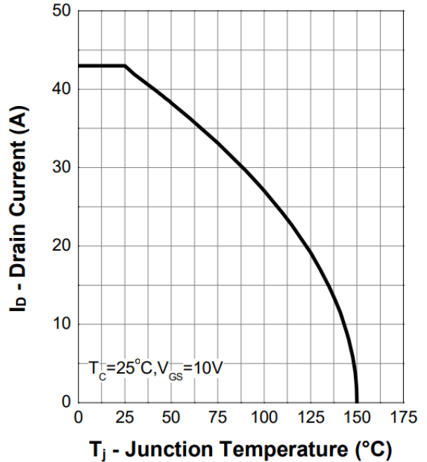
Figure 2. Current Capability
