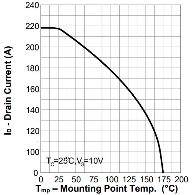
Figure 2. Current Capability
