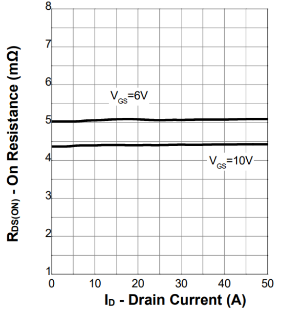
Figure 6. On-Resistance
