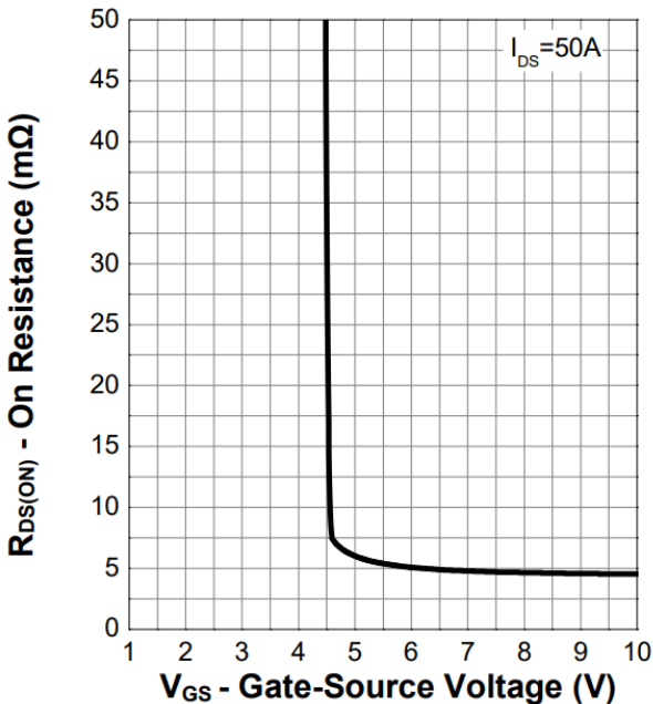
Figure 7. Transfer Characteristics
