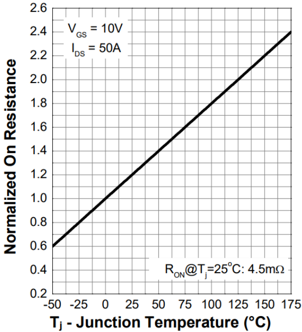
Figure 9. Normalized On-Resistance
