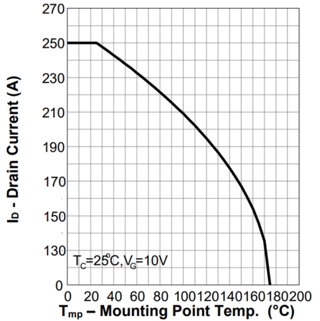
Figure 2. Current Capability
