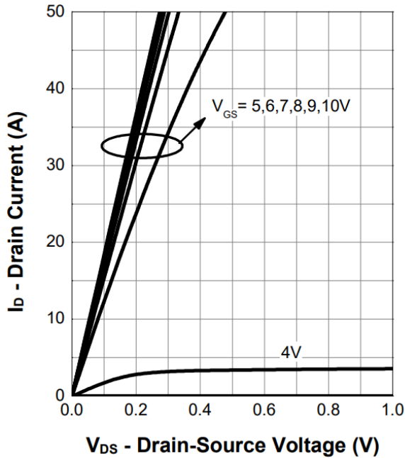
Figure 5. Output Characteristics
