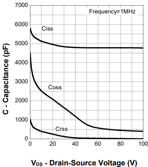
Figure 11. Capacitance
