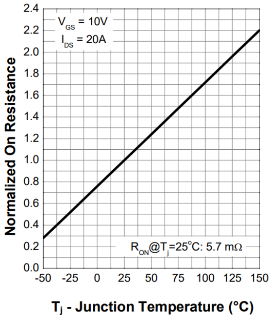
Figure 9. Normalized On-Resistance
