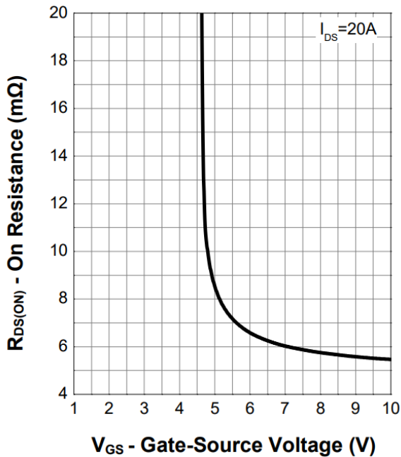
Figure 7. Transfer Characteristics
