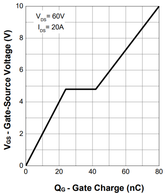
Figure 12. Gate Charge
