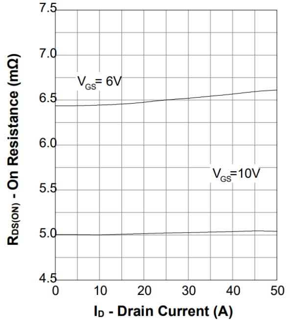
Figure 6. On-Resistance
