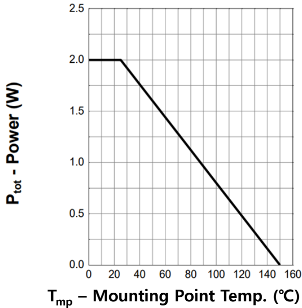
Figure 1. Power Capability
