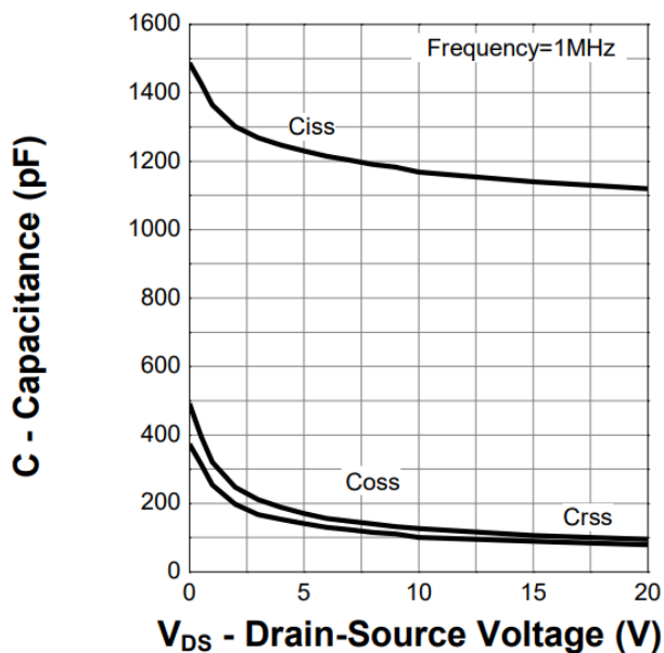
Figure 11. Capacitance
