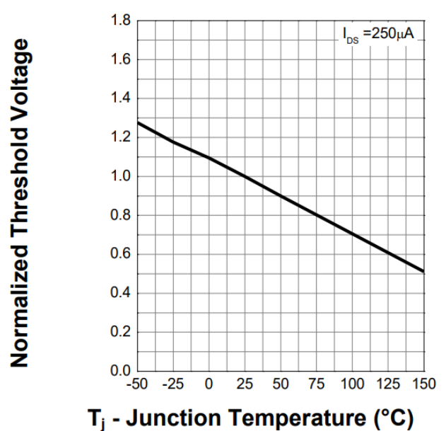
Figure 8. Normalized Threshold Voltage
