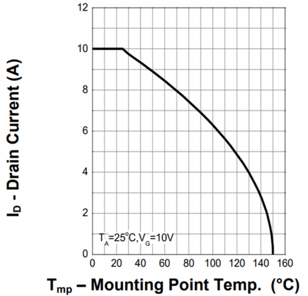
Figure 2. Current Capability
