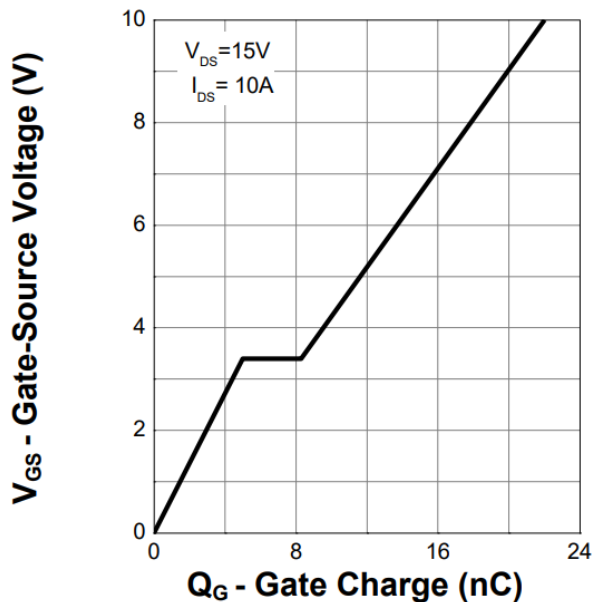
Figure 12. Gate Charge
