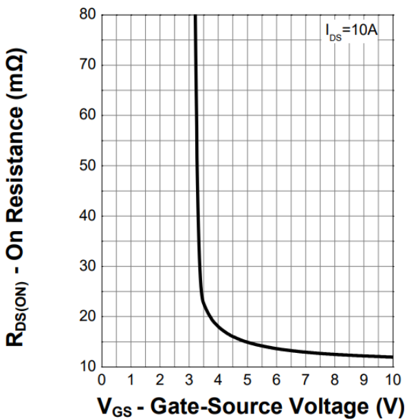
Figure 7. Transfer Characteristics
