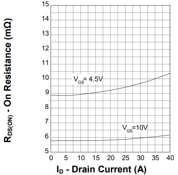
Figure 6. On-Resistance
