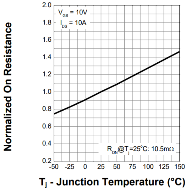
Figure 9. Normalized On-Resistance
