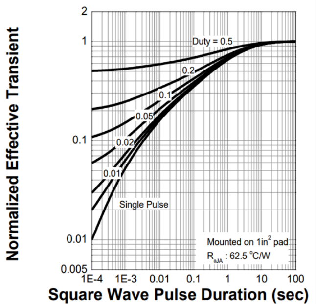
Figure 4. Transient Thermal Impedance
