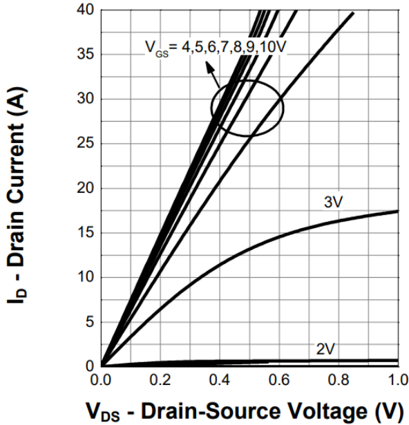
Figure 5. Output Characteristics
