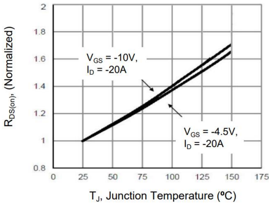
Figure 7. Drain-Source On-Resistance
