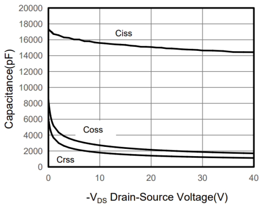
Figure 5. Capacitance
