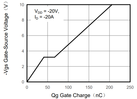
Figure 4. Gate Charge
