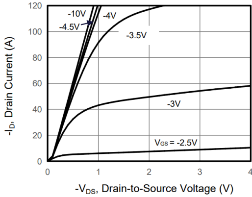
Figure 1. Output Characteristics
