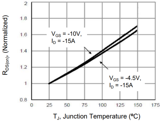
Figure 7. Drain-Source On-Resistance
