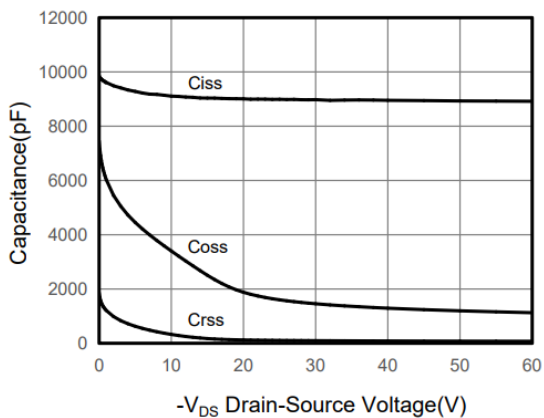
Figure 5. Capacitance
