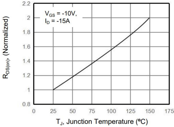
Figure 7. Drain-Source On-Resistance
