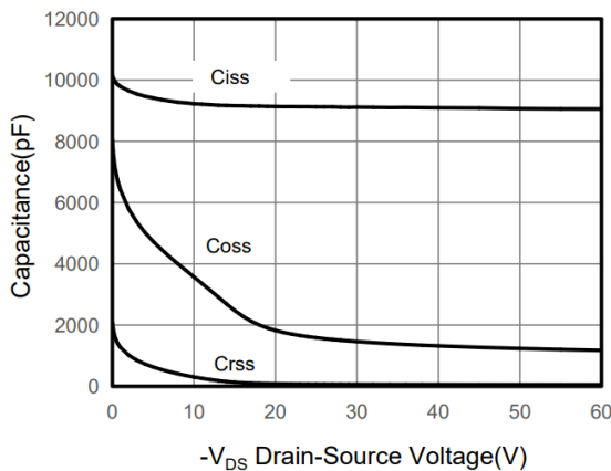
Figure 5. Capacitance
