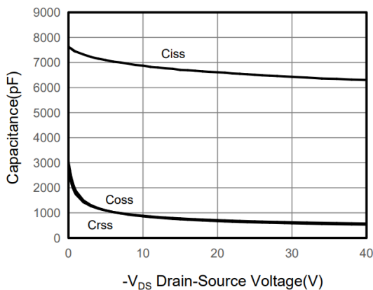
Figure 5. Capacitance
