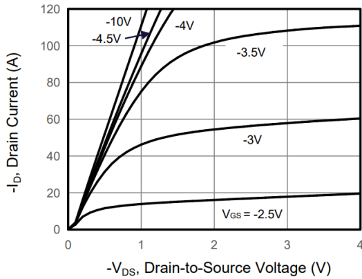
Figure 1. Output Characteristics
