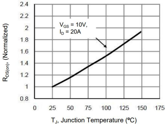
Figure 7. Drain to Source On-Resistance
