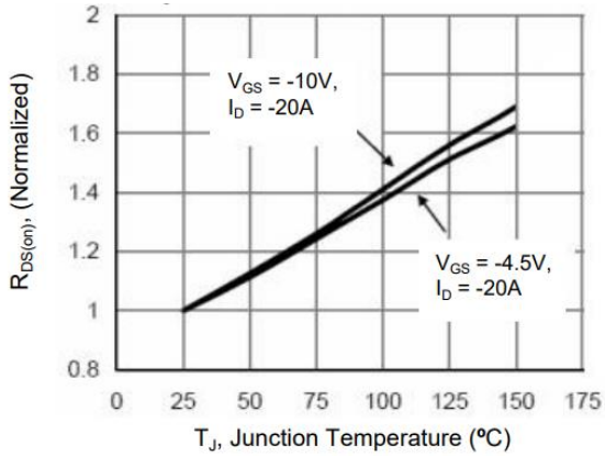
Figure 7. Drain-Source On-Resistance
