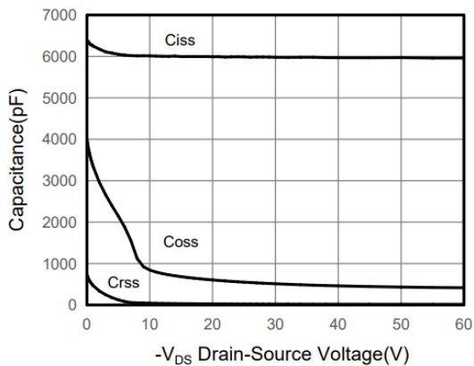
Figure 5. Capacitance
