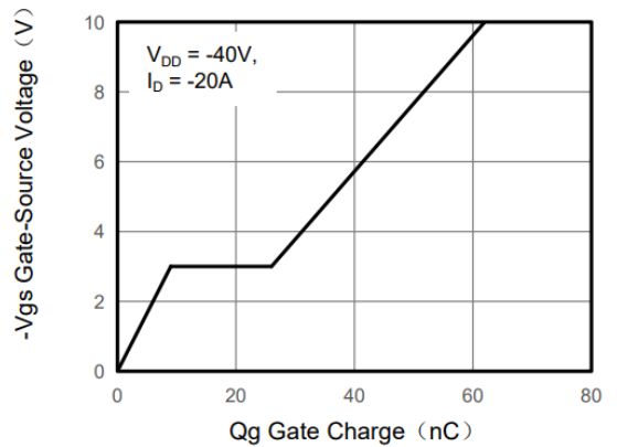
Figure 4. Gate Charge
