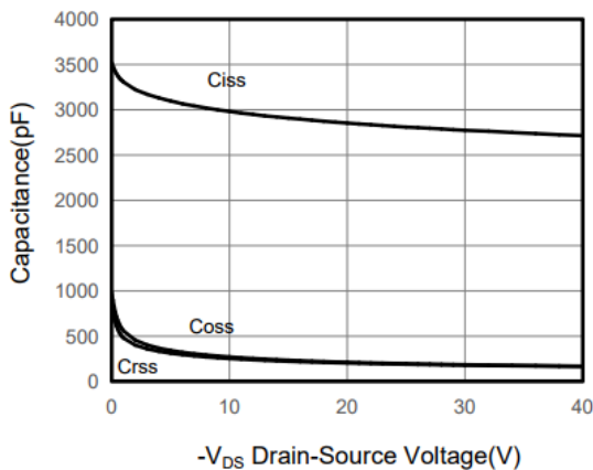
Figure 5. Capacitance
