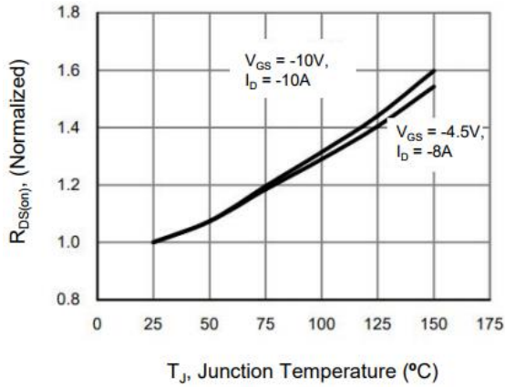
Figure 7. Drain-Source On-Resistance
