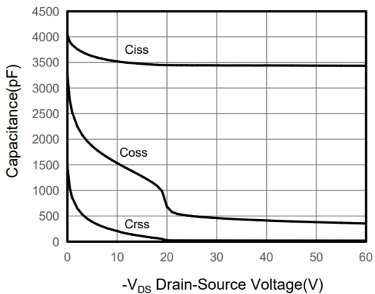
Figure 5. Capacitance
