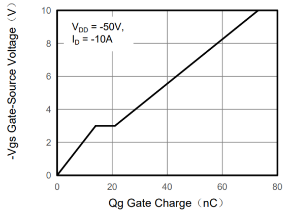
Figure 4. Gate Charge
