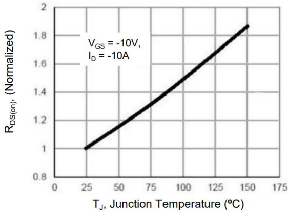
Figure 7. Drain-Source On-Resistance
