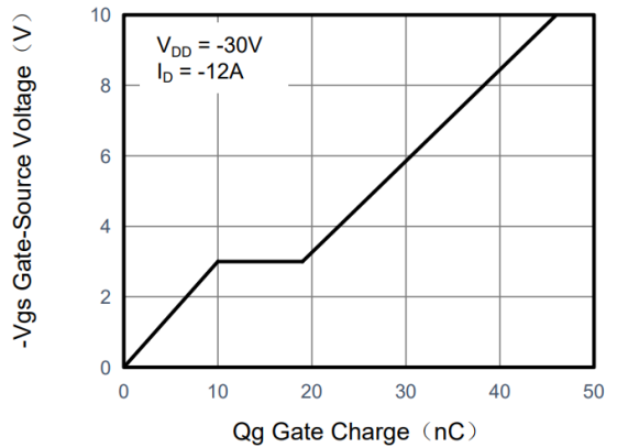
Figure 4. Gate Charge
