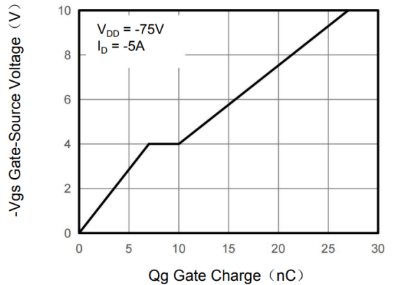
Figure 4. Gate Charge
