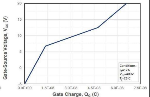
Figure 16. Gate Charge Characteristics
