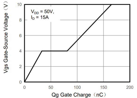
Figure 4. Gate Charge
