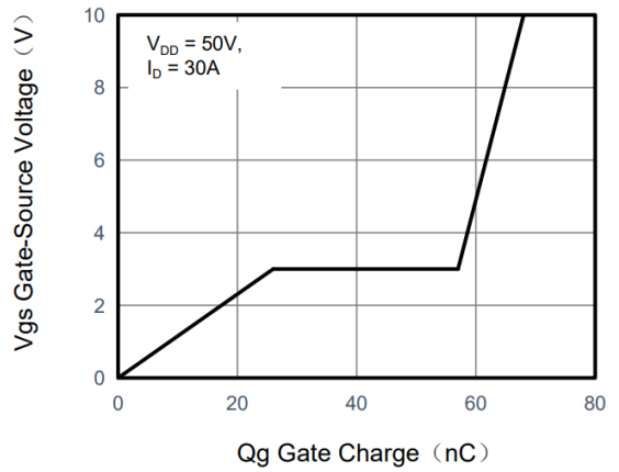
Figure 4. Gate Charge
